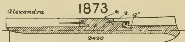
PLATE VI. THE DISTRIBUTION OF ARMOR.
